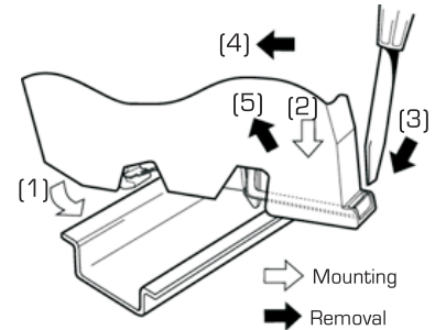
Figure 1 - Mounting/removing a SLP unit
